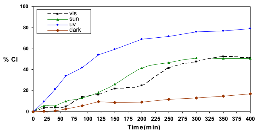
Figure 7 Cl% formed versus time through the catalytic photodegradation process of chlorpyrifos in distilled water.
