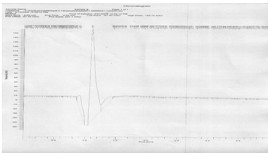
Figure 5 HPLC chromatogram of chlorpyrifos (5 ppm).
