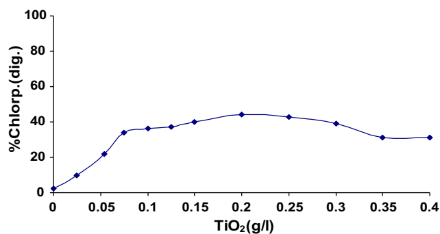
Figure 3 Effect of catalyst loading on the catalytic photodegradation of 5 ppm of chlorpyrifos.
