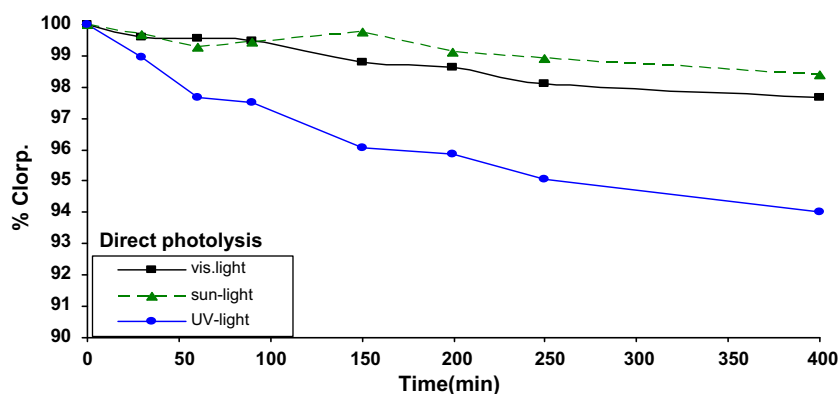
Figure 2 Direct photodegradation of chlorpyrifos under different types of radiation.
