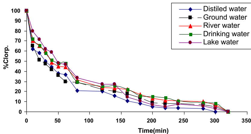
Figure 9 Catalytic photodegradation of chlorpyrifos under UV light radiation in different types of water.
