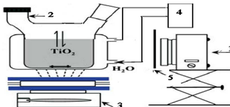
Figure 1 Block diagram of photodegradation reactor 1-sources of light 2-photochemical thermostat cell 3-stirrer 4-recycle water bath (water circulation).
