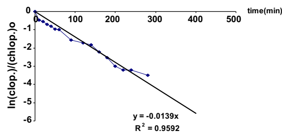
Figure 6 Plotting of \ln [\text{clorp}]/[\text{clorp}]_0 versus time of catalytic photodegradation over \text{TiO}_2/\text{UV} in distilled water.
