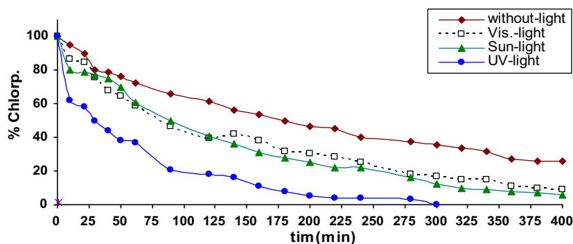
Figure 4 Catalytic photodegradation of chlorpyrifos under different types of radiation.
