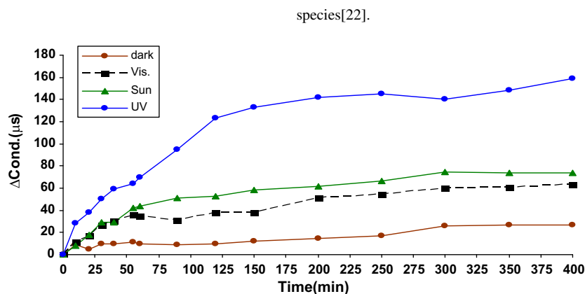
Figure 8 Conductivity changing versus time of through the catalytic photodegradation process of chlorpyrifos in distilled water.
